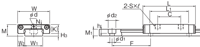
RSR3~7WM/WN型
