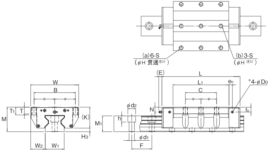
SRG100LC形
